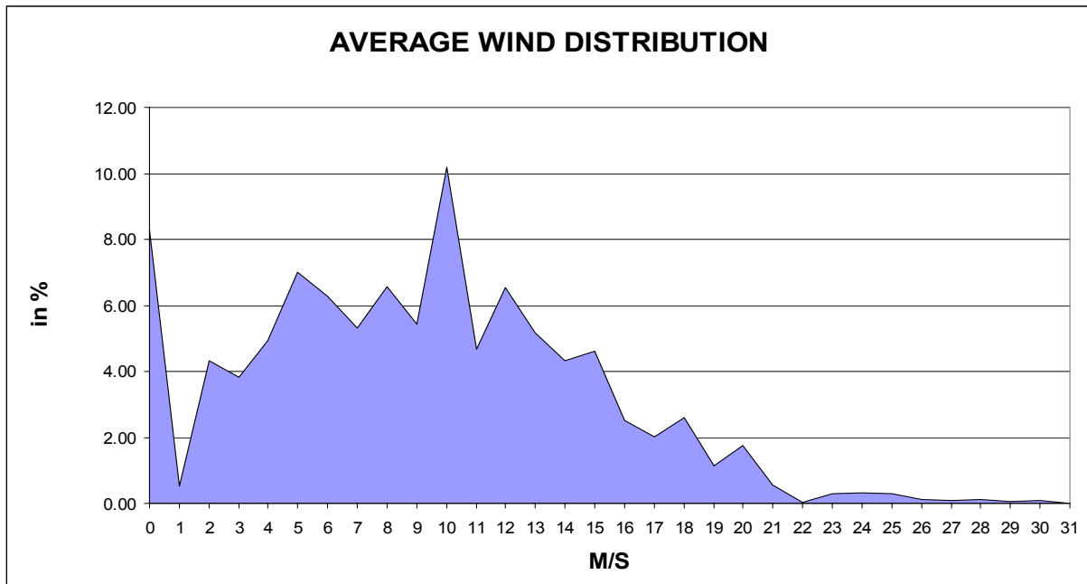
Figure 5 - Average wind distribution
