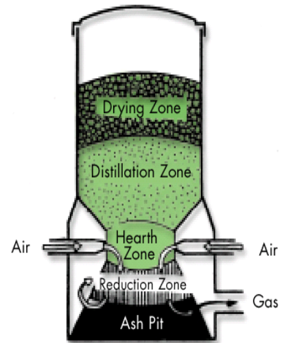
Schematic of Downdraft Gasifier.
